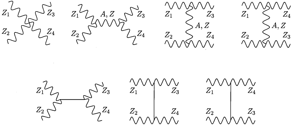
FIG. 5. Diagrams contributing to the scattering process Z_L Z_L \rightarrow Z_L Z_L in NC U(1) \times U(1) ; the subscripts denote the momentum carried by the field.
