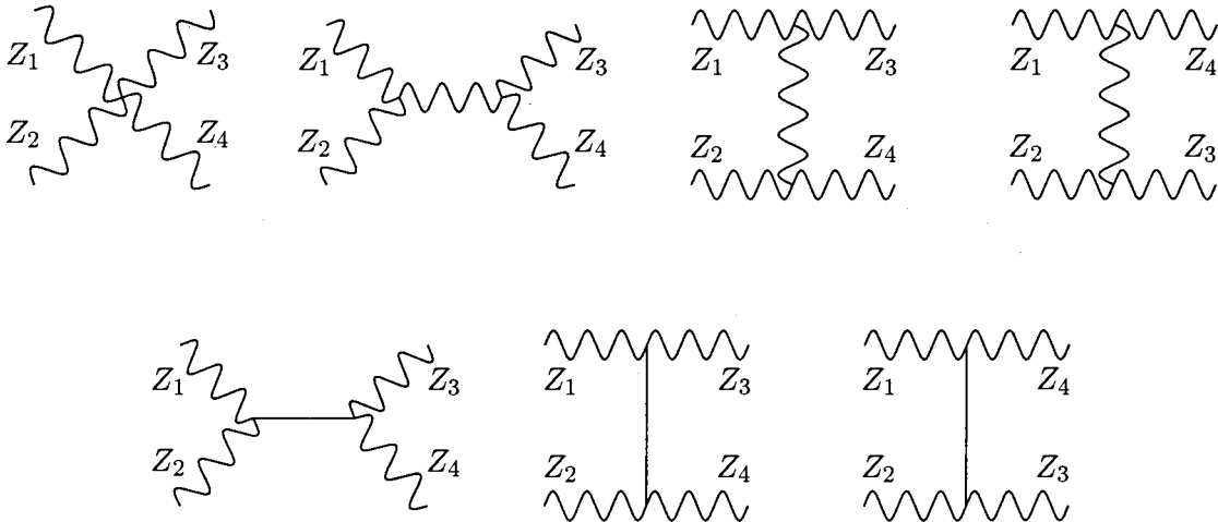
FIG. 3. Diagrams contributing to the scattering process Z_L Z_L \rightarrow Z_L Z_L in NC U(1) ; the subscripts denote the momentum carried by the field.
